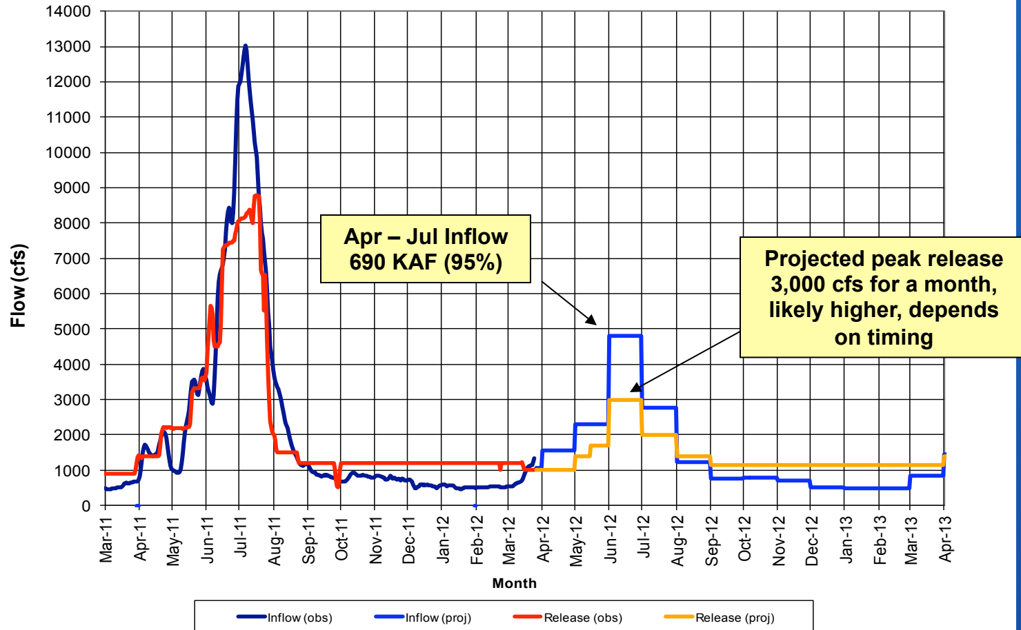
Fontenelle Inflow and Release 2012 Most Probable Operations (Mid-March Forecast)
