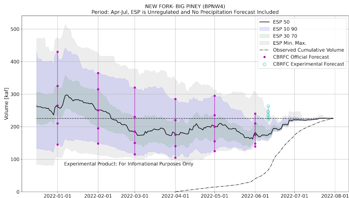
Figure 20: In this data sparse region in the Upper Green River Basin, ASO provided information that led to a more accurate forecast.
