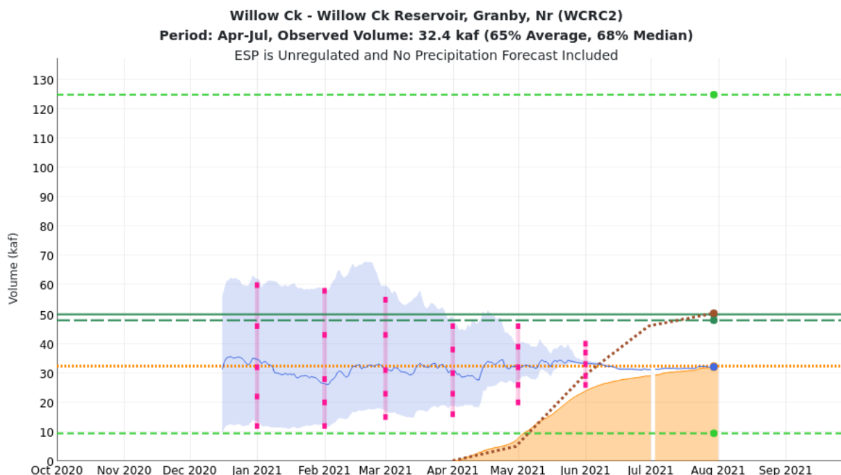
Figure 13: Seasonal water supply forecasts over the Willow Creek watershed after the East Troublesome Fire performed well after changes to parameters within the CBRFC's hydrologic model to account for post-fire impacts.
