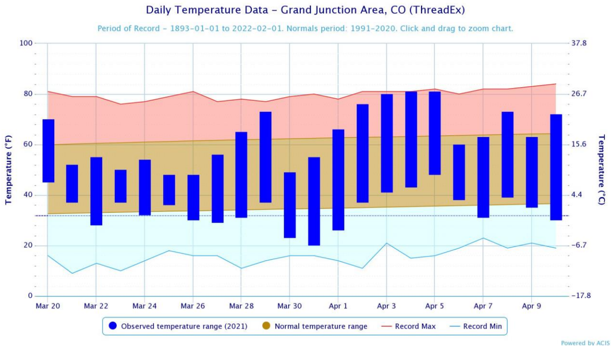
Figure 7: Near record temperatures in the Colorado River Basin contributed to early season melt of below normal snowpack conditions. Here, near record temperatures in early April are shown in the Grand Junction, CO area.
